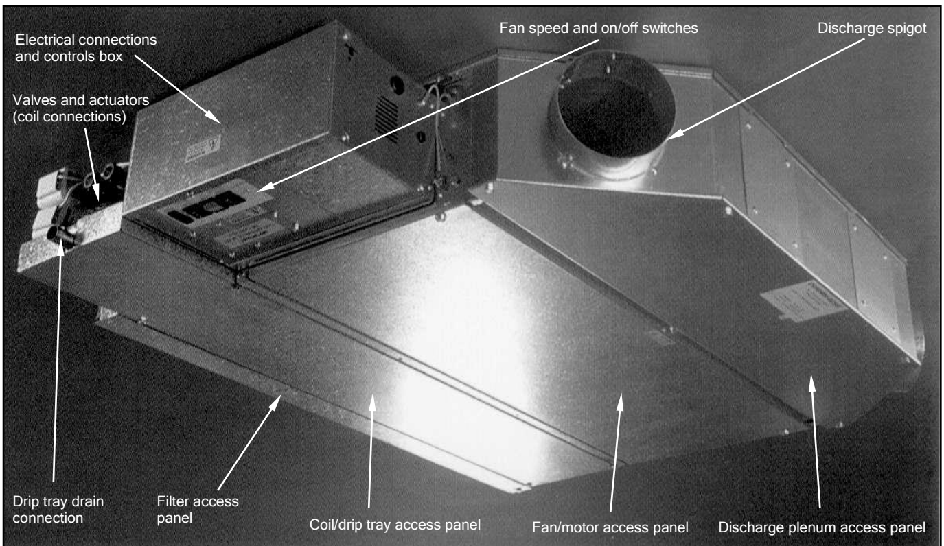
Diagram 1 - Cougar Fig 3 LH connections with octagonal discharge plenum
