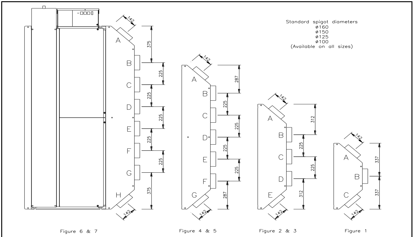
Diagram 4: Standard spigot sizes and positions
