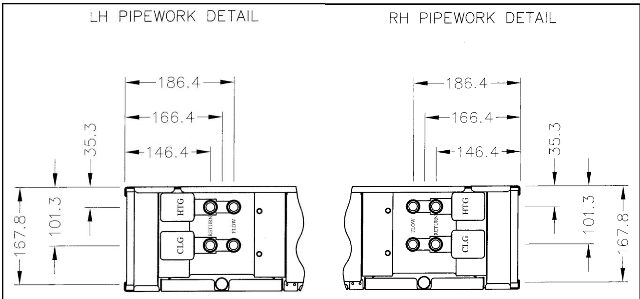
Diagram 5: Pipework connections, as viewed on header/connection end of coil
