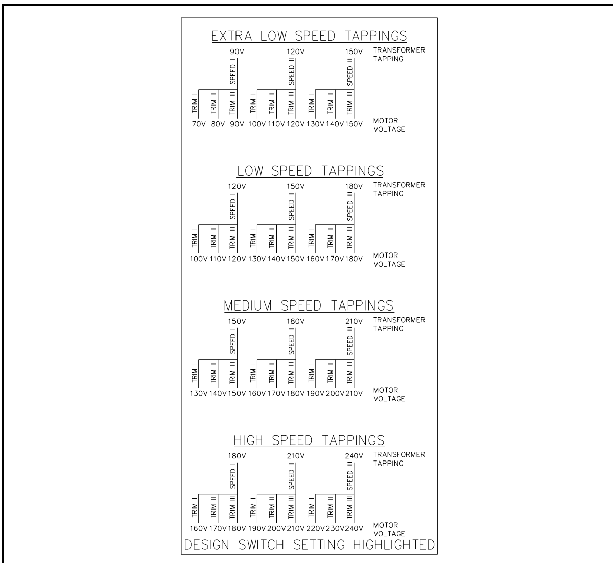
Diagram 8: Fan switch speed settings; also shown as label affixed to fan coil unit (AC motor units only)
