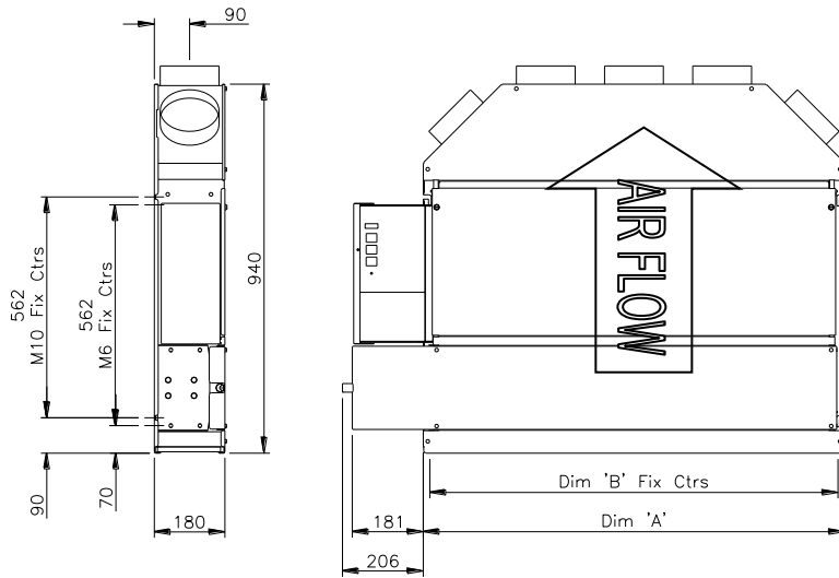
Diagram 2: Range of standard sizes with octagonal discharge plenum
